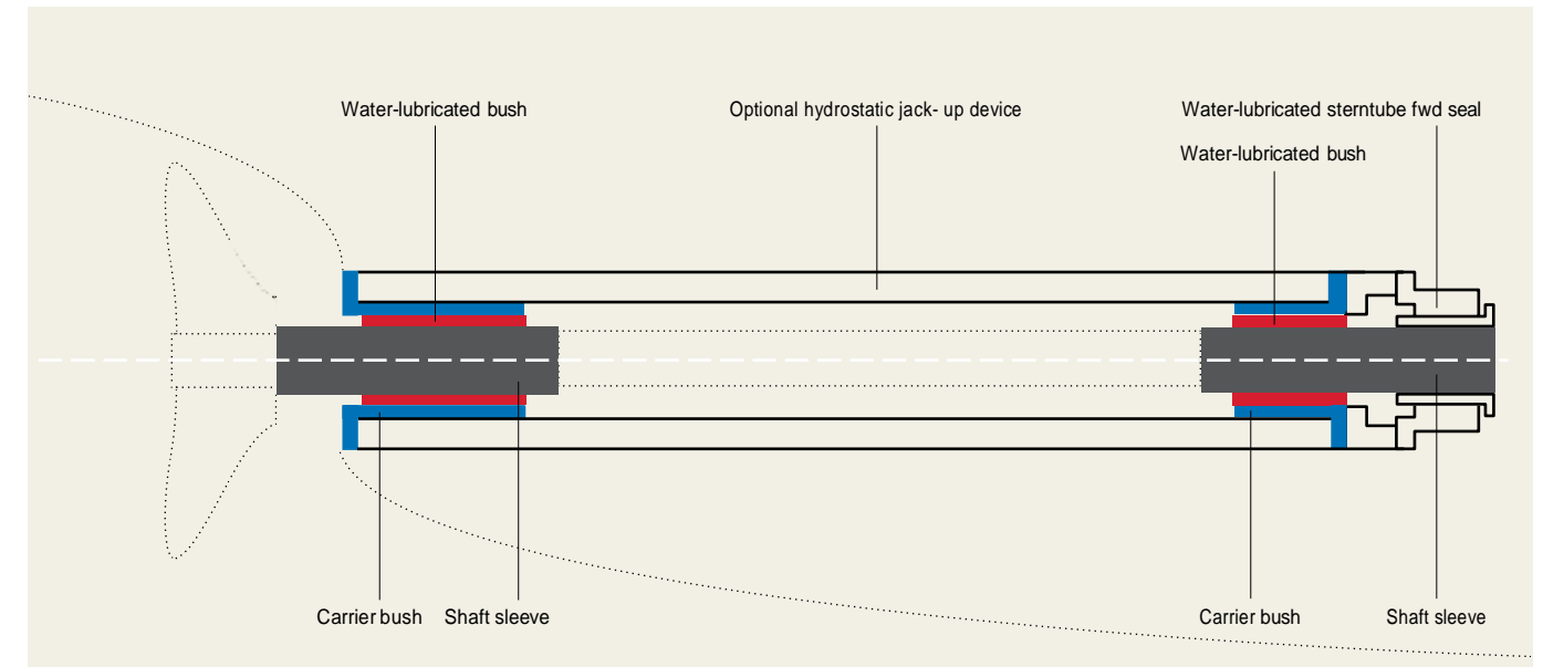
Type 2: Open water lubricated sterntube system
