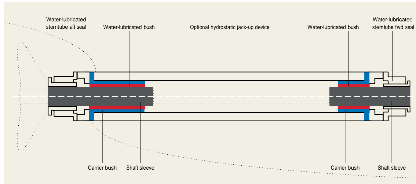
Type 1: Closed sterntube system with fresh water filling and anti-corrosive protection additive
