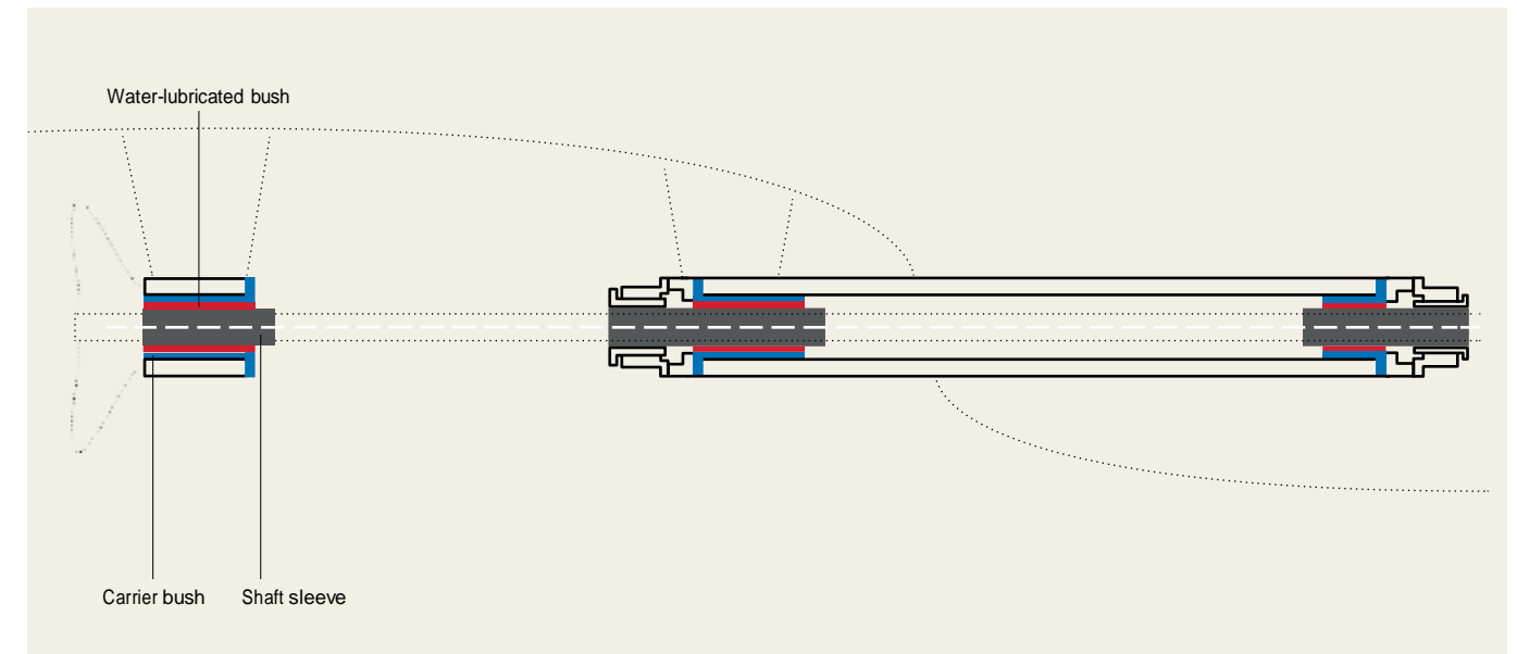
Type 3: Open sea water-lubricated propeller shaft bearings
